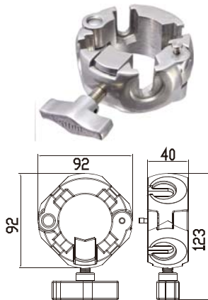
KCP-950P 4 Way Clamp for 35mm to 50mm tube
