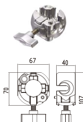
KCP-930P 3 Way Clamp for 25mm to 35mm tube
